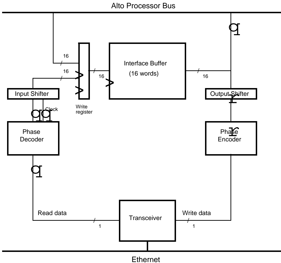
Figure 9 -- Ethernet Control
