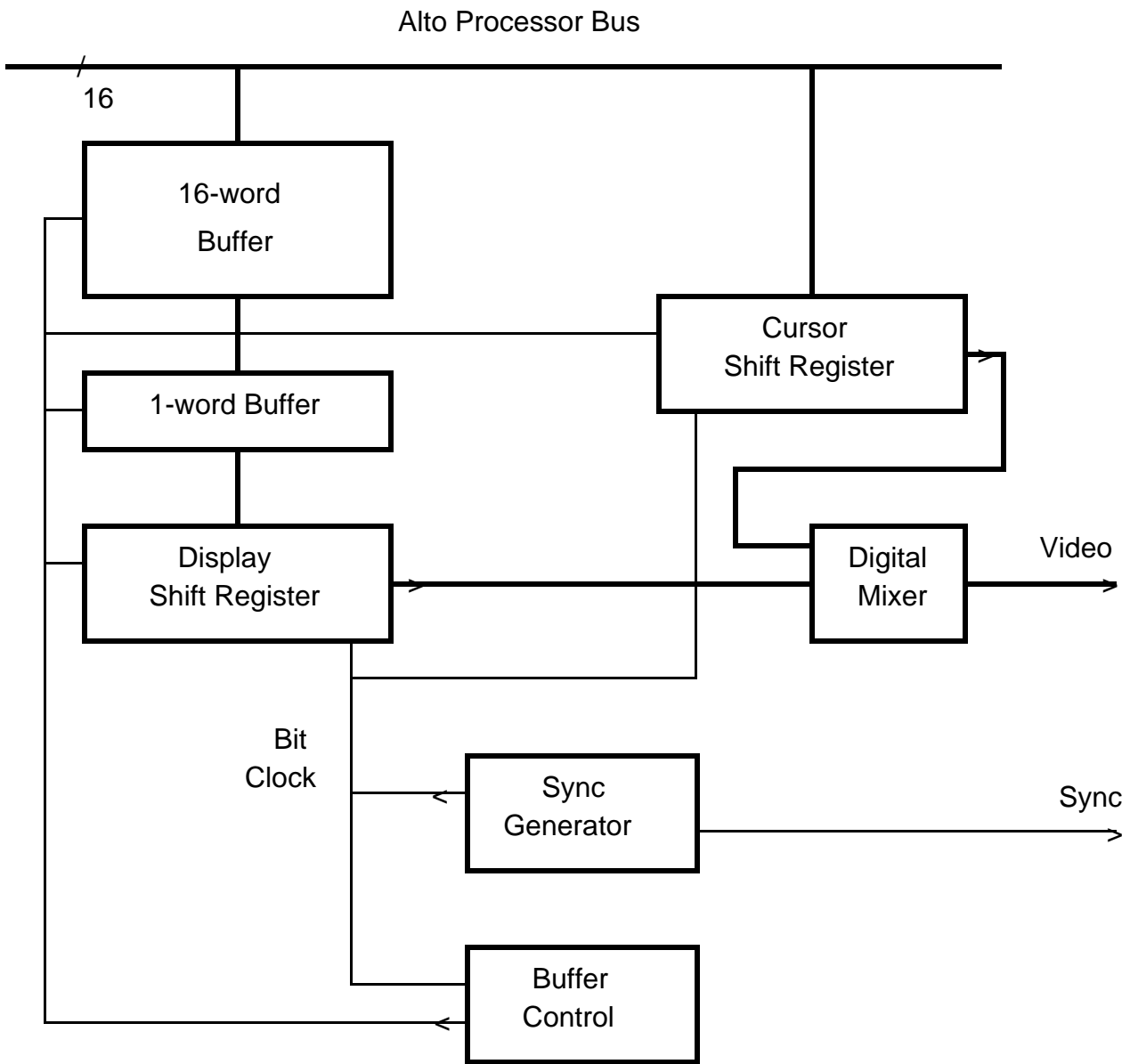
Figure 5 -- Display Control
