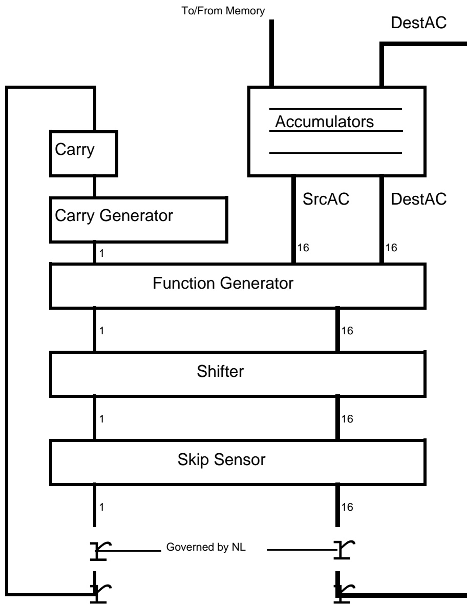
Figure 4 -- Instruction Execution
